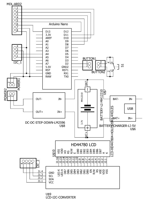
Fig. 4. Circuit
