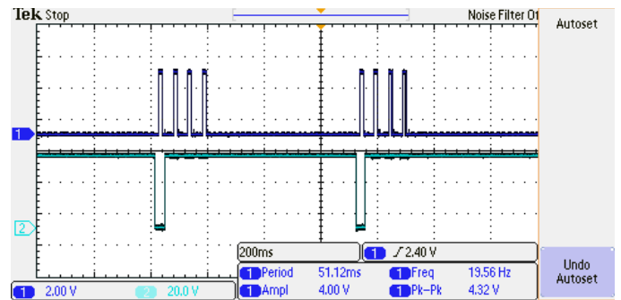
Fig. 16. Measurement results on SO and CS pins in module 1
