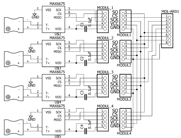
Fig. 3. Circuit
