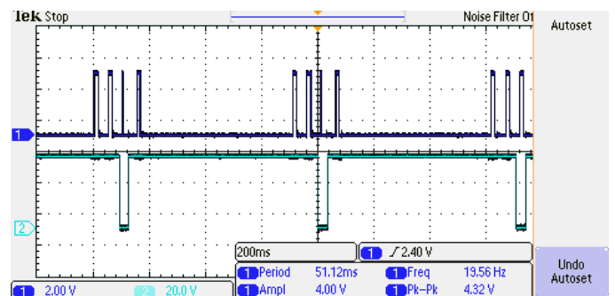
Fig. 18. Measurement results on SO and CS pins in module 3
