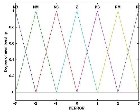
FIGURE 5. Membership Function Delta Error
