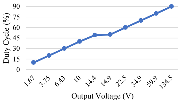
FIGURE 7. Graph of output voltage to duty cycle
