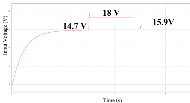
FIGURE 10. Input Voltage Waveform on Pico Hydro Power Plant System
