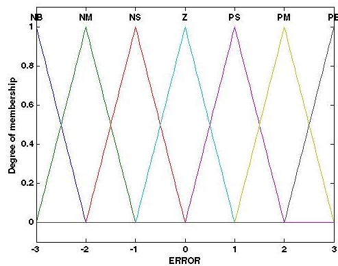
FIGURE 4. Error Membership Function
