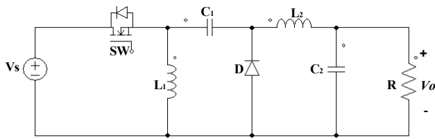
FIGURE 2. The Circuit of Zeta Converter
