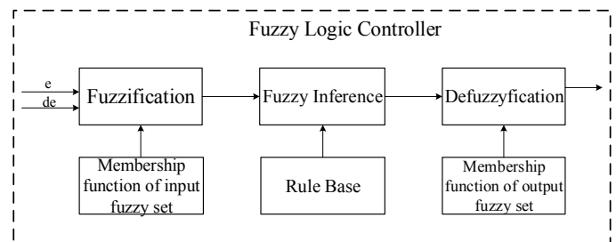
FIGURE 3. Block Diagram of Fuzzy Logic Controller
