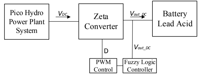
FIGURE 1. The Diagram Block of Pico Hydro Power Plant
