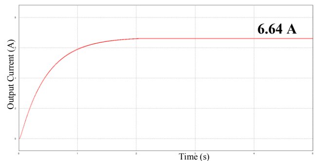
FIGURE 9. Output Current Simulation Waveform on Pico Hydro Power Plant System using FLC
