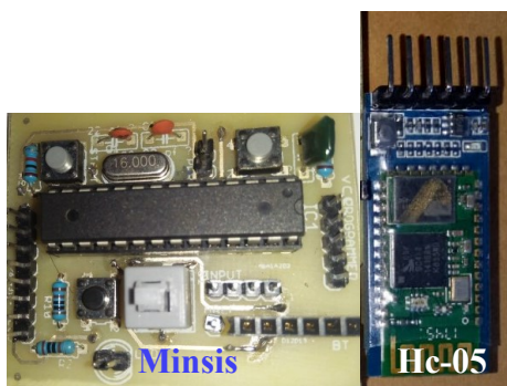
Fig. 8. The digital part of the design Respiration Rate
