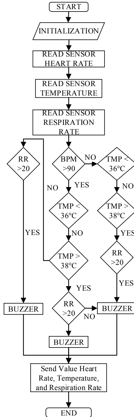
Fig. 2. The flowchart of the Arduino Program
