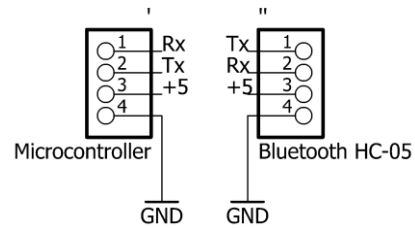
Fig. 5. Bluetooth Connection
