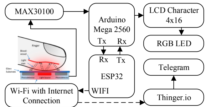
FIGURE 1 Diagram Block
